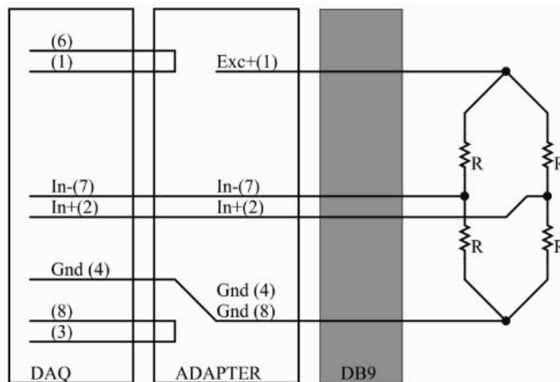
Illustration 14: BRIDGE-F- 2.5V Full bridge
