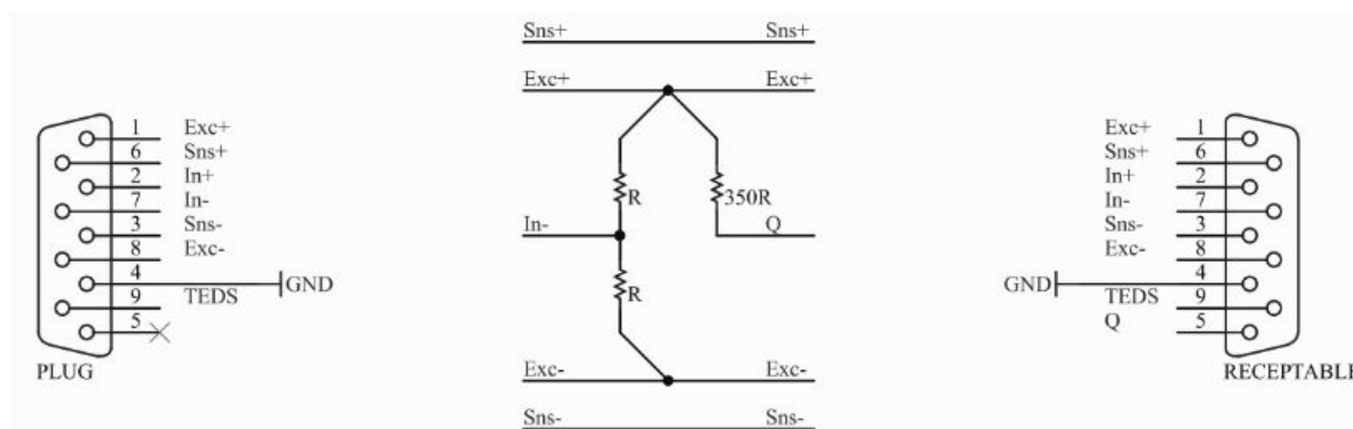
Illustration 1: BRIDGE-QH-350-10V Schematics
