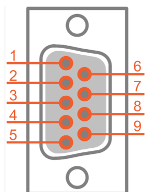
Illustration 12: Input connector (DSUB 9pin) pinout
