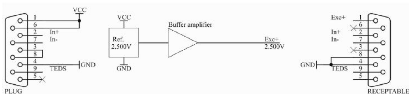
Illustration 11: BRIDGE-F- 2.5V Schematics
