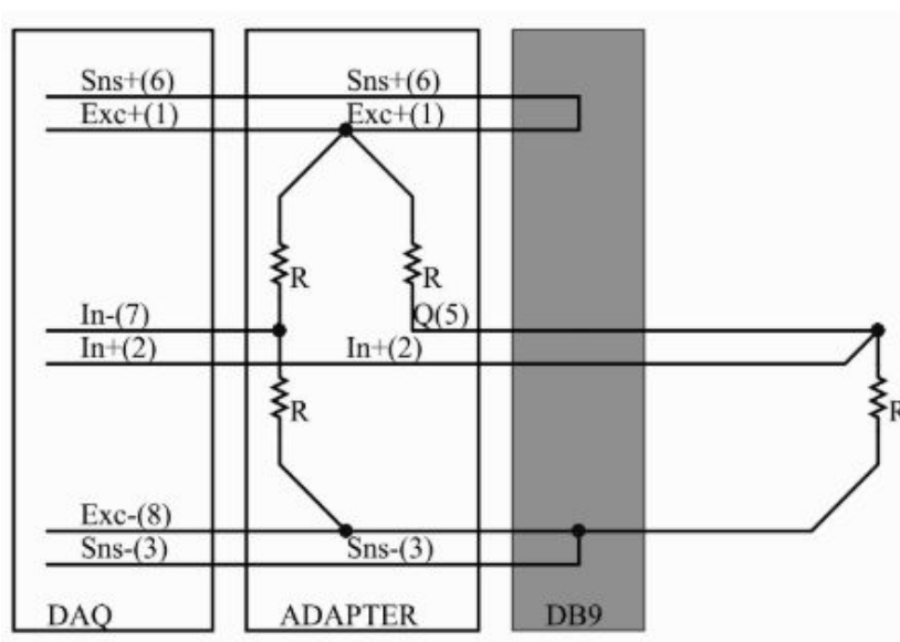
Illustration 5: BRIDGE- QH- 350- 10V 3- wire Quarter bridge
