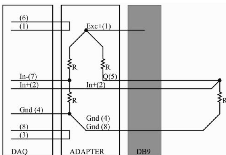
Illustration 10: BRIDGE- QH- 120- 2. 5V, BRIDGE-QH-350-2. 5V 3- wire Quarter bridge
