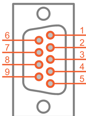
Illustration 13: Output connector (DSUB 9pin) pinout
