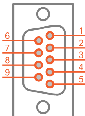
Illustration 3: Output connector (DSUB 9 connector) pinout
