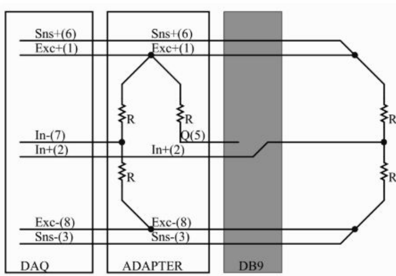
Illustration 4: BRIDGE- QH- 350- 10V Half bridge
