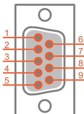
Illustration 7: Input connector (DSUB 9pin) pinout
