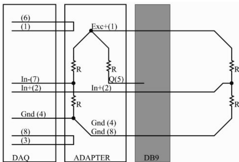
Illustration 9: BRIDGE- QH- 120- 2. 5V, BRIDGE-QH-350-2.5V Half bridge
