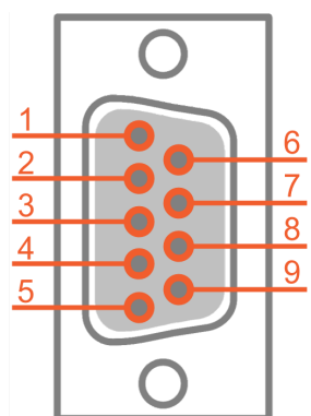
Illustration 2: Input connector (DSUB 9 connector) pinout
