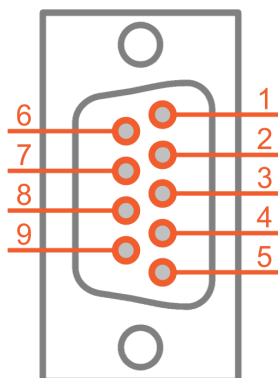
Illustration 8: Output connector (DSUB 9pin) pinout
