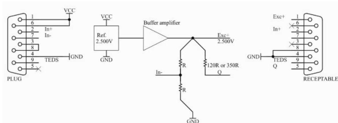
Illustration 6: BRIDGE- QH- 120- 2. 5V, BRIDGE-QH-350-2. 5V Schematics
